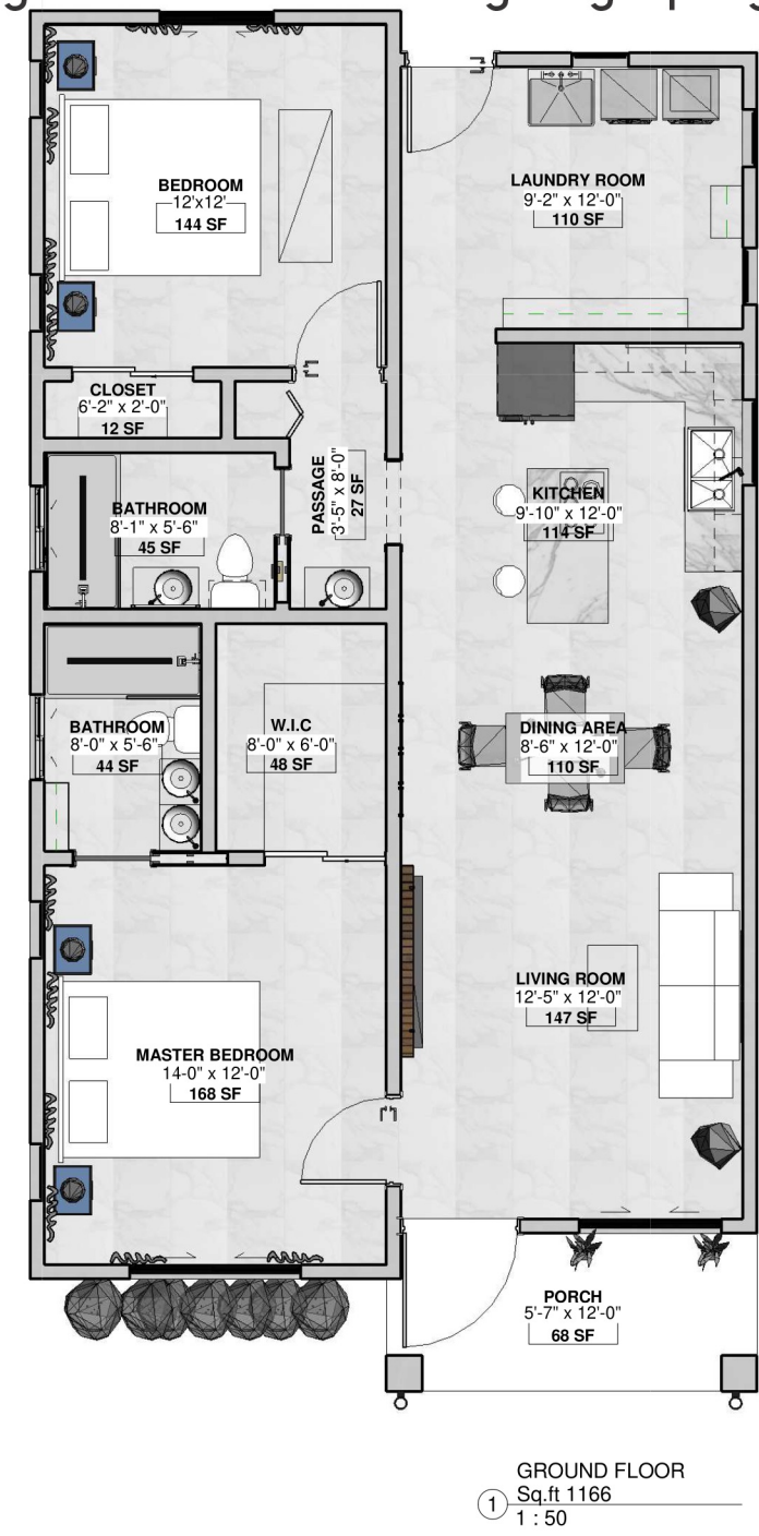
TWIN PALM FLOOR PLAN- 1166 Sq. ft. Fig. 2 without covered garage/pergola
