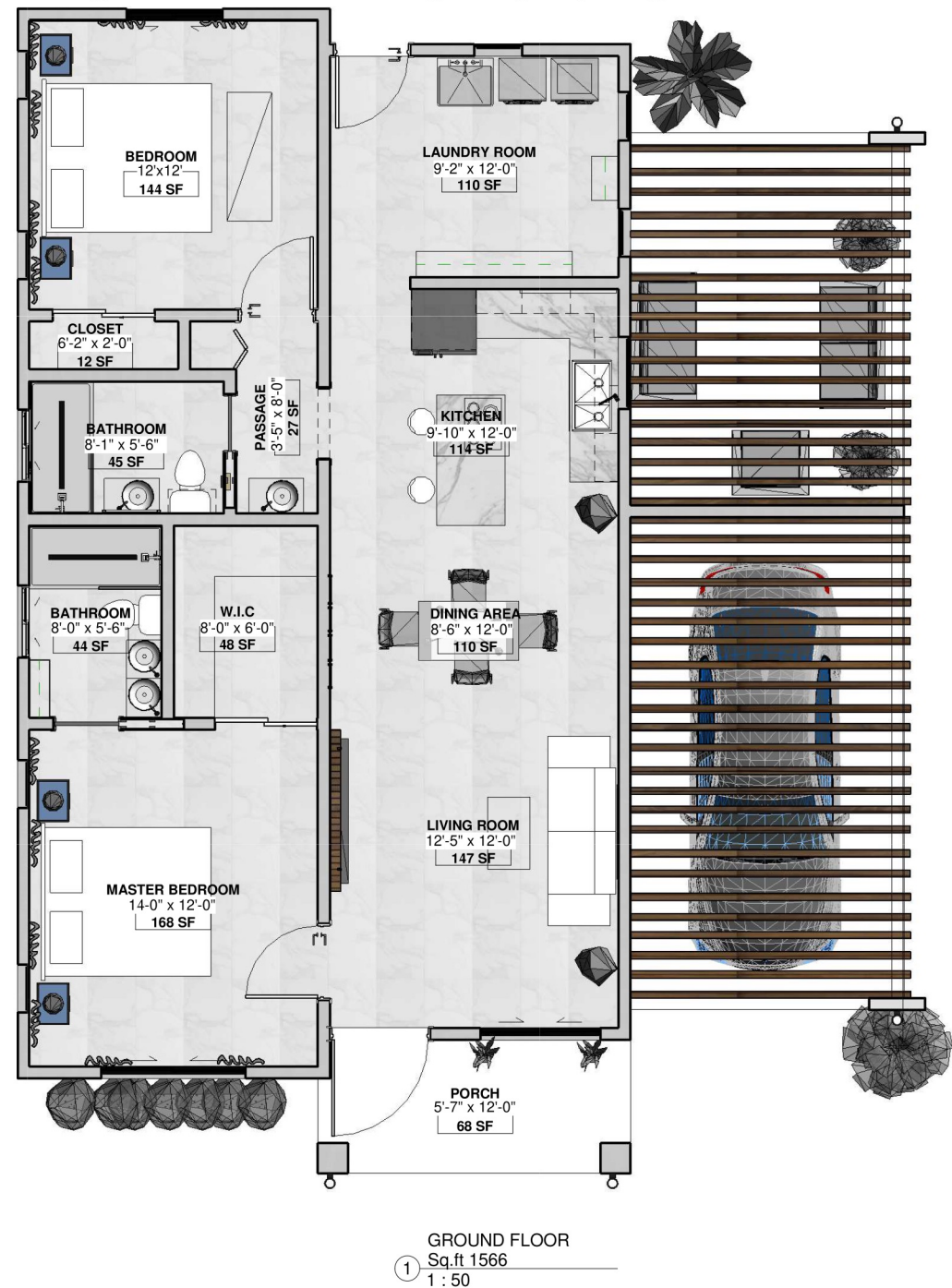
TWIN PALM FLOOR PLAN- 1566 Sq. ft. Fig. 1 with covered garage/pergola
